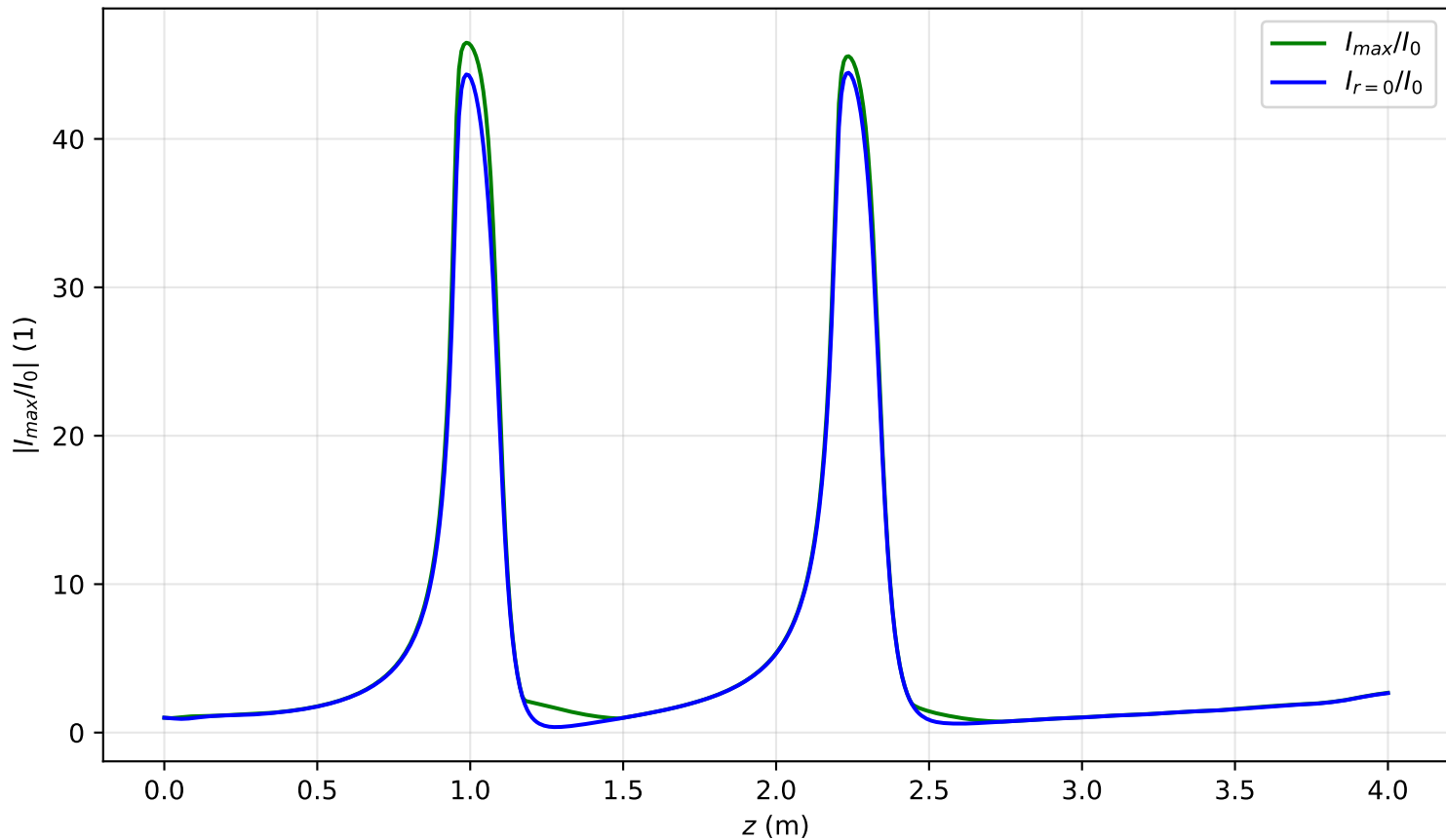
I_{max}(x=0, y=0, z)/I_0 , P_{in}=2.3P_{cr} , noisy input, artificial time
